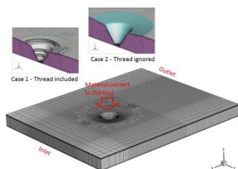
Figure 24. FSW process CFD computer model.
