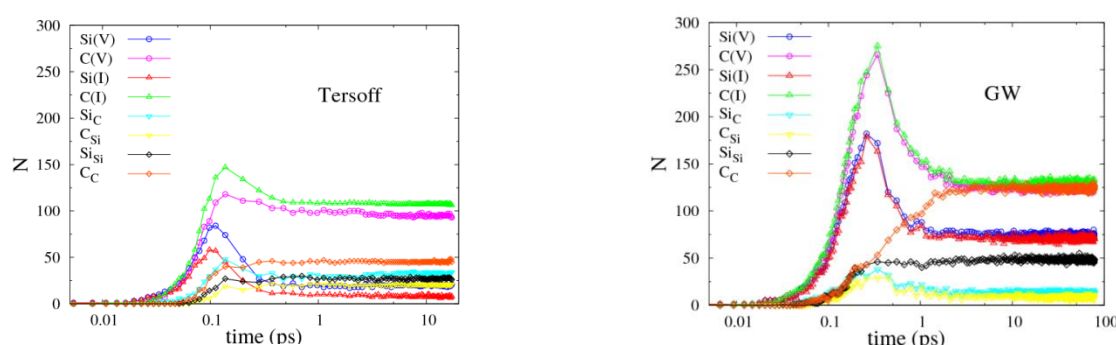
Figure 72. Time dependence of the number of point defects observed in MD displacement cascade simulations at 10 keV pka at 300 K: (a) Tersoff potential, (b) GW potential.
