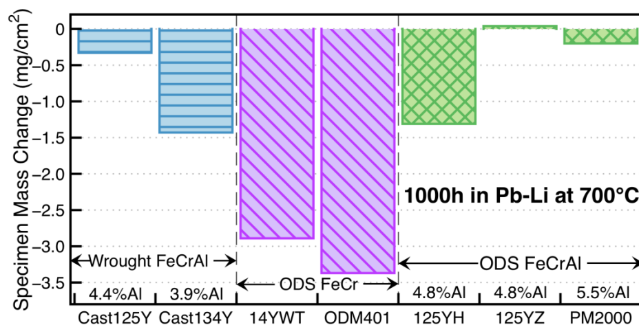
Figure 13. Specimen mass change for alloy specimens exposed for 1000 h at 700°C in static Pb-Li.
