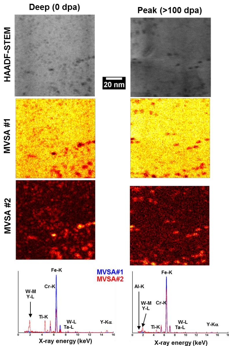
Figure 19. Left column, unirradiated. Right column, near-peak irradiated ( \sim 1500 nm depth, >100 dpa). HAADF: high-angle annular dark field. MVSA: multivariate statistical analysis.
