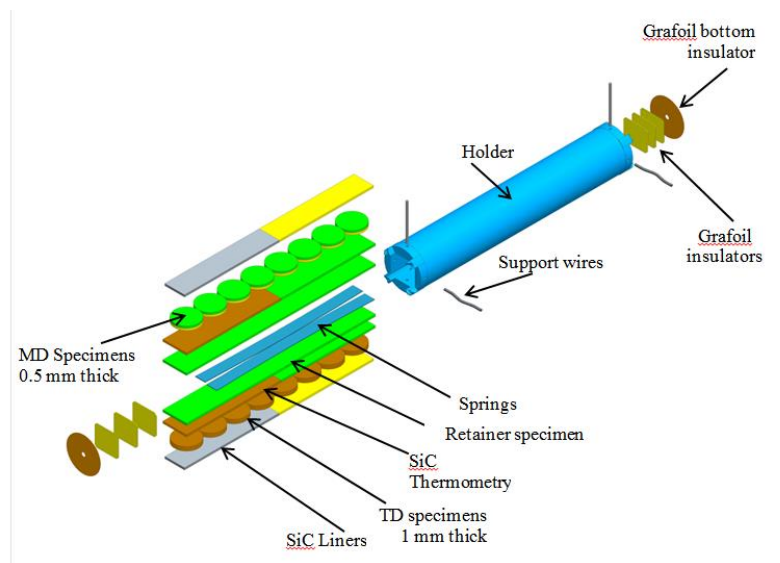
Figure 84. Exploded PRO/E View of the PXW Rabbit Tungsten Rabbit Inner Assembly
