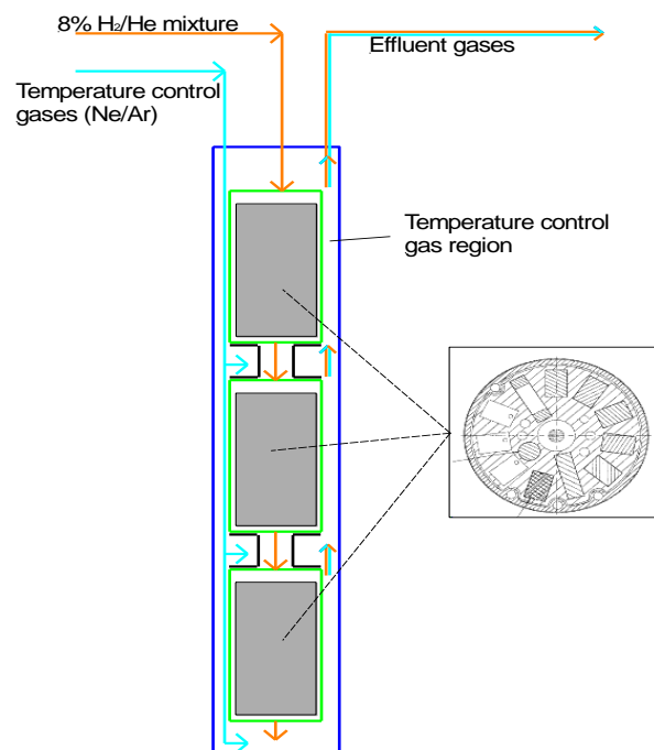
Figure 80. Gas Flow Diagram of the Capsule
