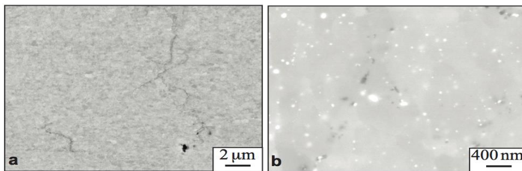
Figure 8. SEM backscattered electron images of (a) 125YT after extrusion and (b) 125YH after annealing for 1000h at 800°C
