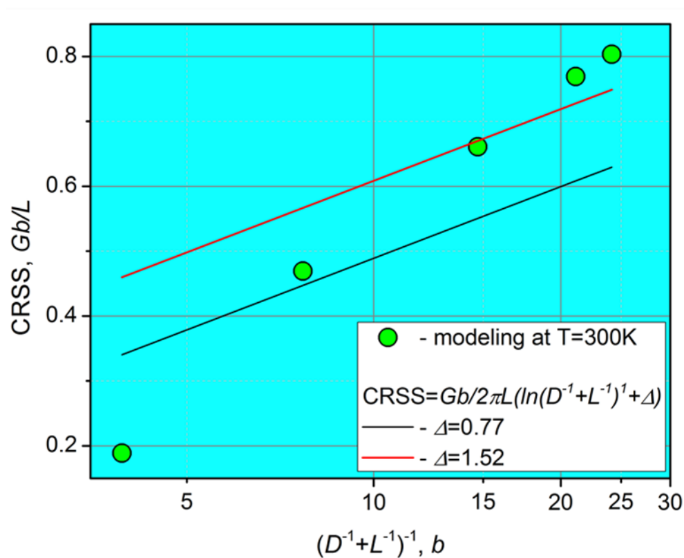
Figure 79. Critical resolved shear stress in reduced units as a function of harmonic mean of an obstacle diameter, D, and spacing between them along the dislocation line. Circle - rigid inclusions simulated in current work, lines are dependences obtained in dislocation dynamic modeling for Orowan mechanism (black line) and void (red line) in [1,2].
