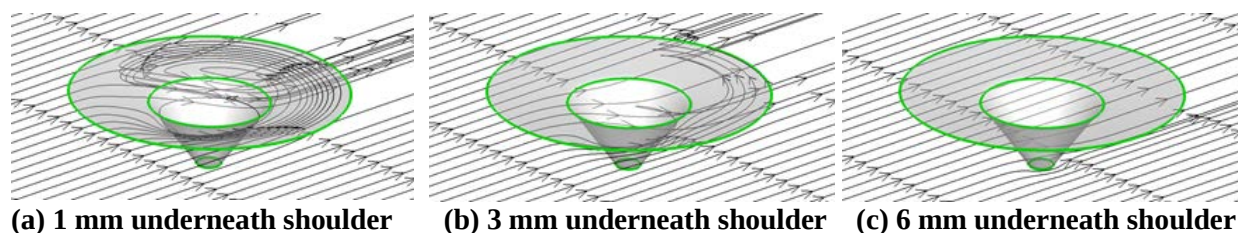
Figure 22. Flow pattern predictions by CFD computer modeling (Advancing side on the right).
