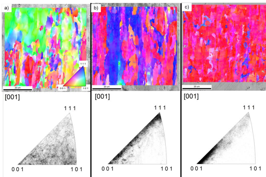
Figure 44. EBSD analysis of the a) 250 \mu\text{m} thick tungsten foil surface, b) 100 \mu\text{m} thick tungsten foil surface, and c) 25 \mu\text{m} thick tungsten foil surface. Rolling direction is vertical on the page.
