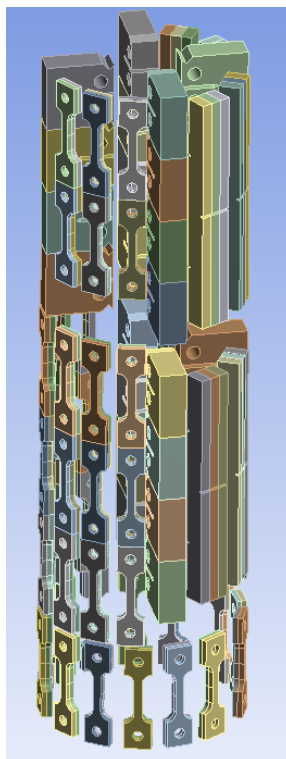
Figure 85. Specimen Design Layout for the 250°C Subcapsule.
