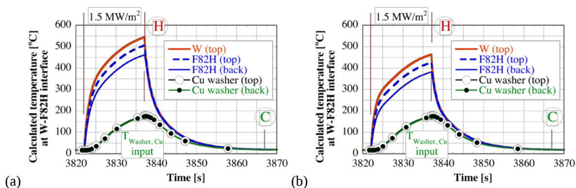
Figure 71. Calculated temperature evolution during cycle 42 for thermal contact conduction per unit area between the F82H and Cu washer of (a) 5,000 and (b) 7,000 [W/m 2 K]. The temperature on the back-surface of the Cu washer was used as input.
