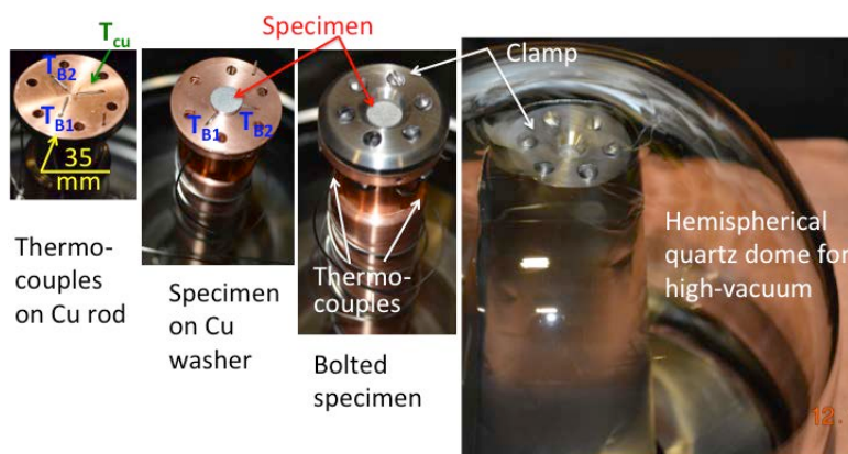
Figure 69. Experimental setup showing the sequence for placing different components. From left to right the individual frames indicate: placement of thermocouples on Cu rod, Cu washer and specimen on the rod, clamping the specimen, thermocouple shield and high-vacuum dome, respectively.
