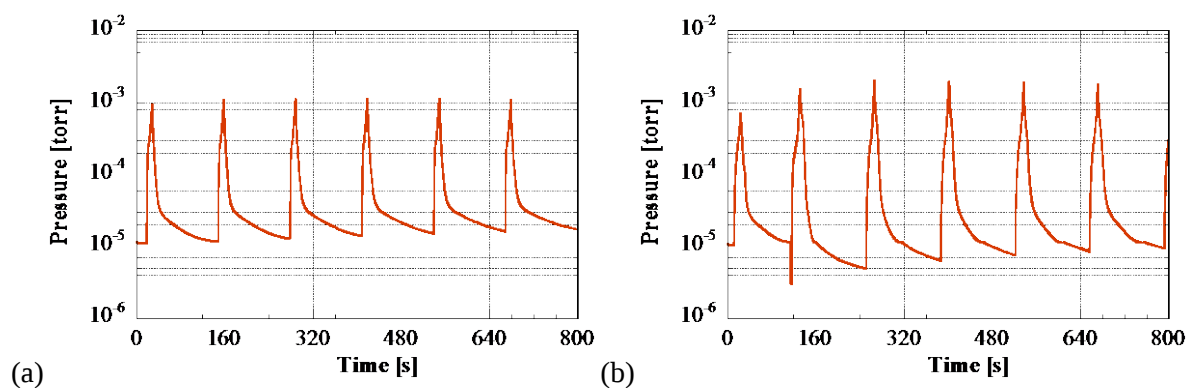
Figure 67. Representative data on absolute pressure for specimen 1 and cycles: (a) 84-89 ( 300 \text{ W/cm}^2 for 10 s) and (b) 132-137 ( 300 \text{ W/cm}^2 for 12 s cycle 132 and 15 s for cycles 133-137).
