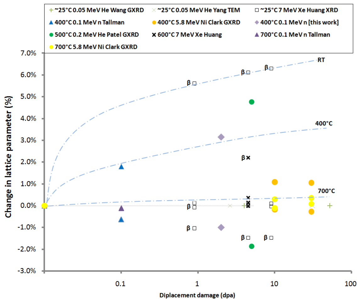
Figure 2. Irradiation induced swelling measured by GXR, TEM or XRD on predominantly \text{Ti}_3\text{AlC}_2 materials. Positive values denote c-axis swelling, while negative values denote the a-axis shrinkage.
