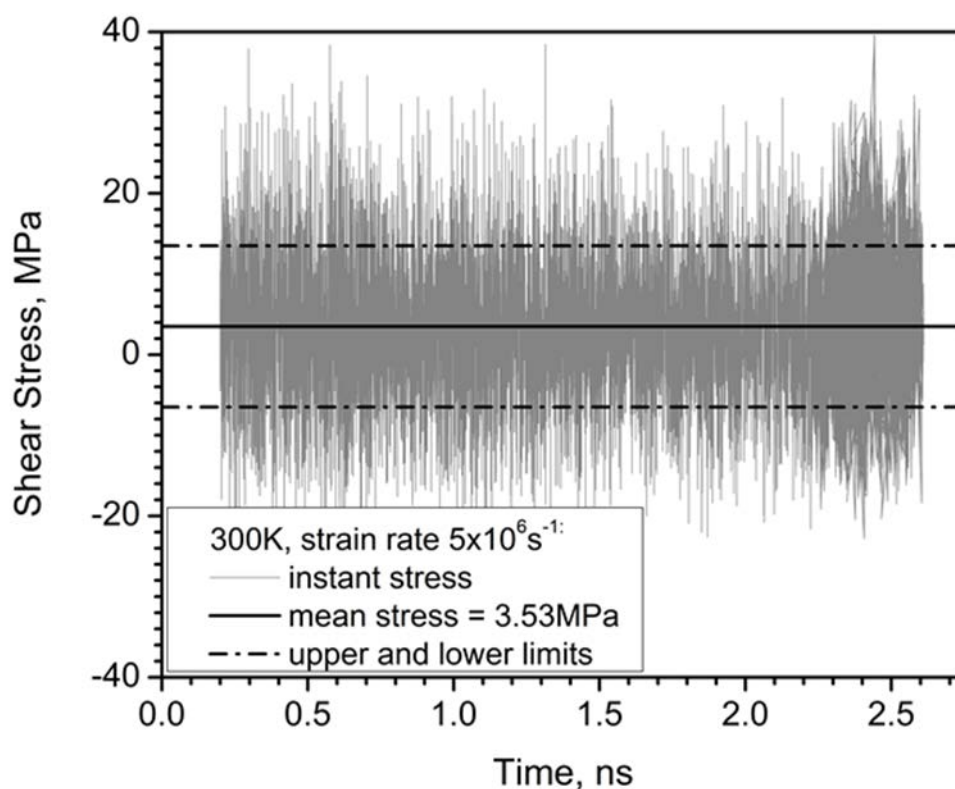
Figure 76. Modeling of steady state motion of \frac{1}{2}\langle 111 \rangle \{110\} dislocation at a strain rate of 5 \times 10^6 \text{ s}^{-1} at 300K: grey line - instantaneous shear stress calculated every 100 time steps ; solid black line - mean value, 3.8 MPa, estimated over 2.5 ns, point-dash lines – mean stress plus/minus standard
