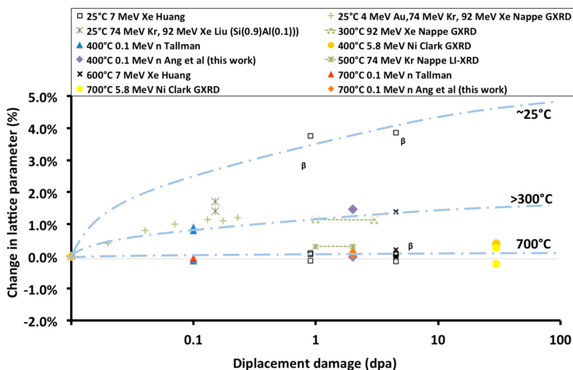
Figure 1. Irradiation induced swelling measured by GXRD (Grazing incidence X-ray Diffraction) or XRD on predominantly \text{Ti}_3\text{SiC}_2 materials. Positive values denote c-axis swelling, while negative values denote the a-axis shrinkage.
