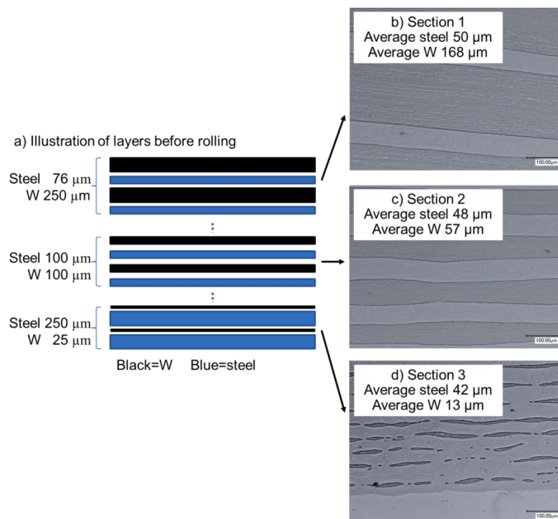
Figure 40. a) Stacking sequence of foils, showing thicknesses before rolling b)-d) SEM images of cross section of laminate after rolling.
