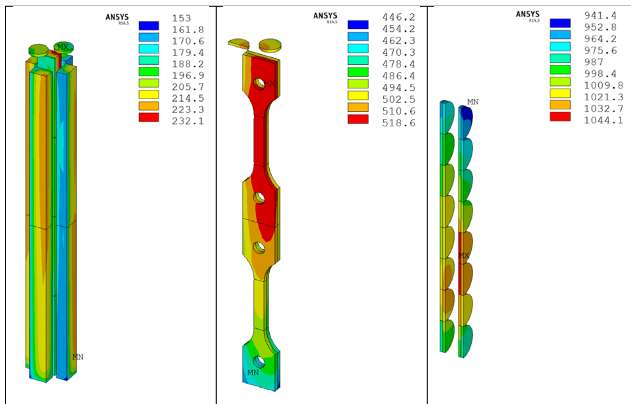
Figure 87. Predicted specimen temperature contours for the 200°C BMG rabbit (left), 500°C HEA rabbit (center, with ½-symmetry), and 1000°C IMR rabbit (right, with ½-symmetry).
